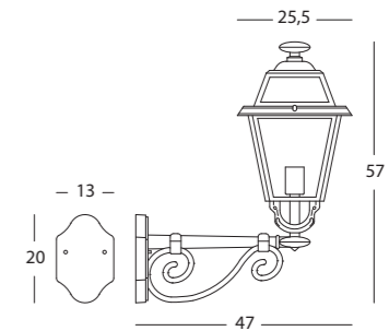
art. 855/16 grigio Lampada H max 210 mm EAN: 8020588221187
