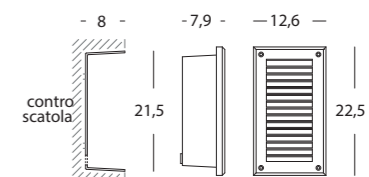
art. 817/16 grigio Lampada H max 125 mm EAN: 8020588937002
