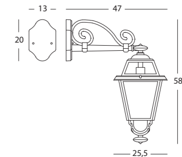
art. 856/16 grigio Lampada H max 210 mm EAN: 8020588221194
