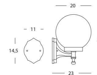
art. 211/06 nero Lampada H max 160 mm. Max 60W EAN: 8020588509063
