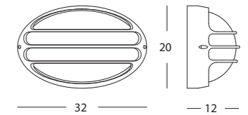
art. 705/16 grigio Lampada H max 170 mm. EAN: 8020588960000
