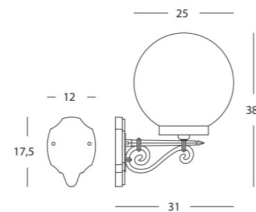
art. 398/06 nero Lampada H max 180 mm. Max 60W EAN: 8020588316067
