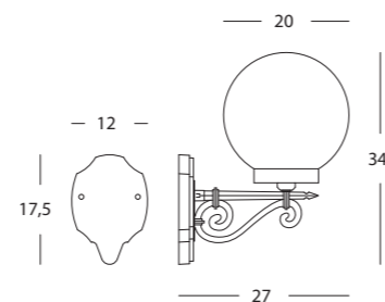
art. 308/06 nero Lampada H max 160 mm. Max 60W EAN: 8020588315060
